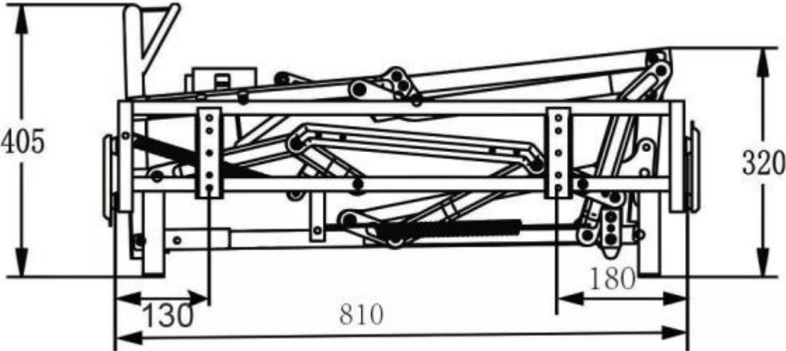
Low Leg Italian Style Sofa Bed Mechanism Mounting & Drawing
